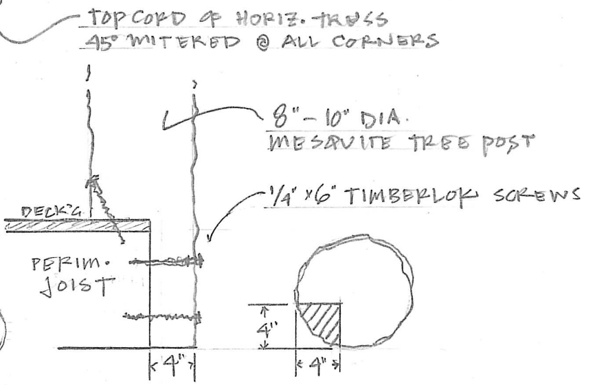
SECTION PLAN 1" = 1'0"
